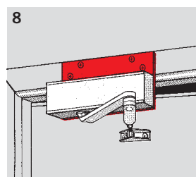
Drop plate installation
