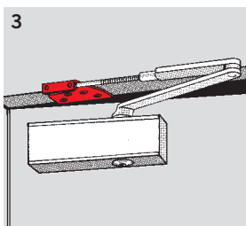
Parallel arm installation
